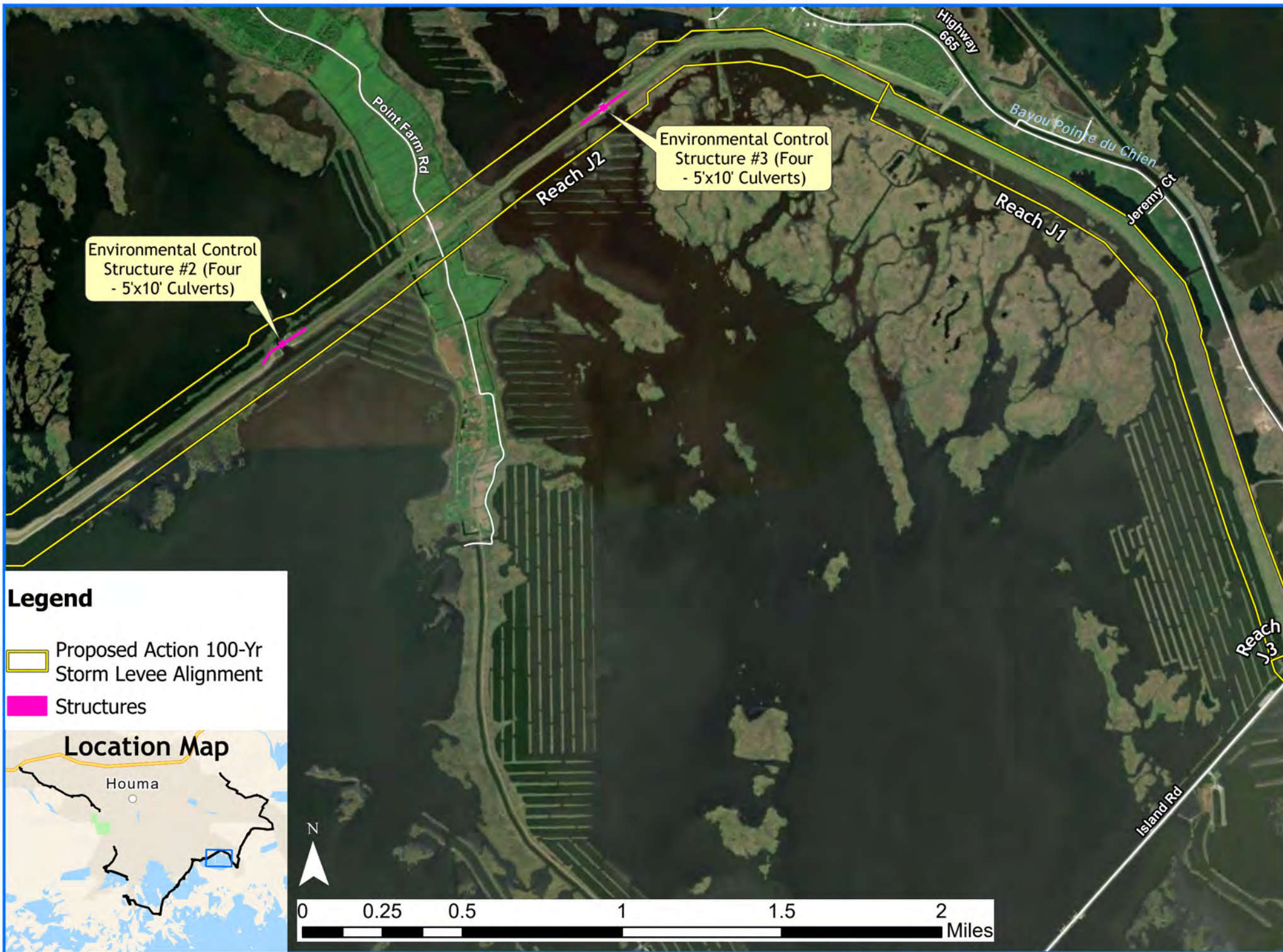
Proposed Action with Structures - Reach J
