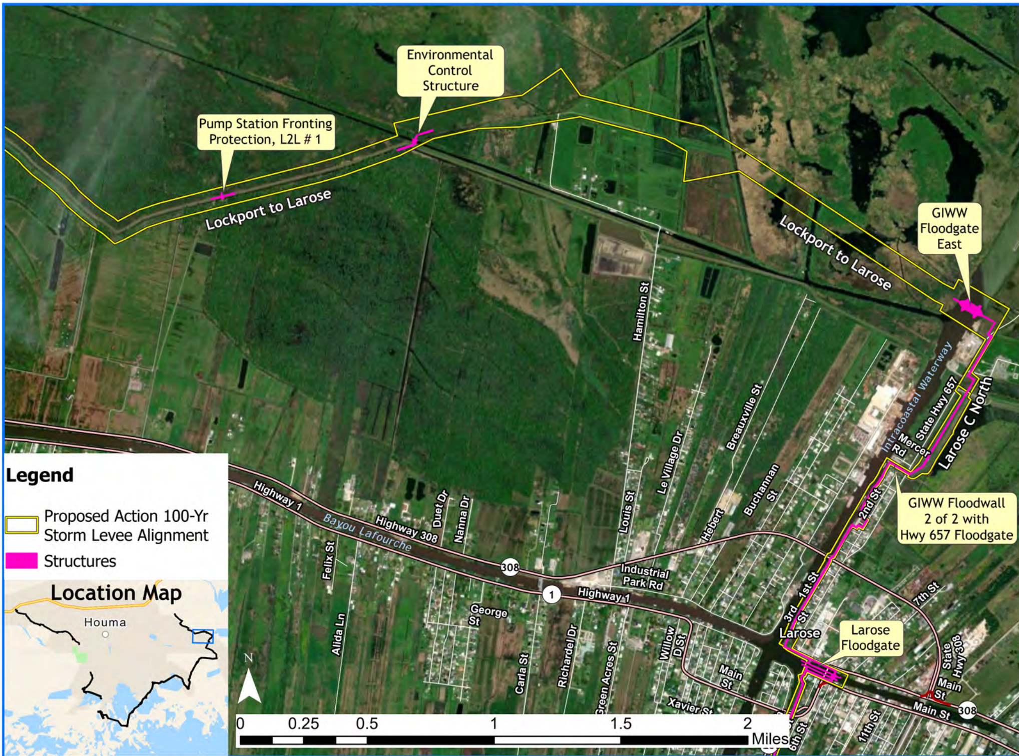
Proposed Action with Structures - Larose C North, Lockport to Larose
