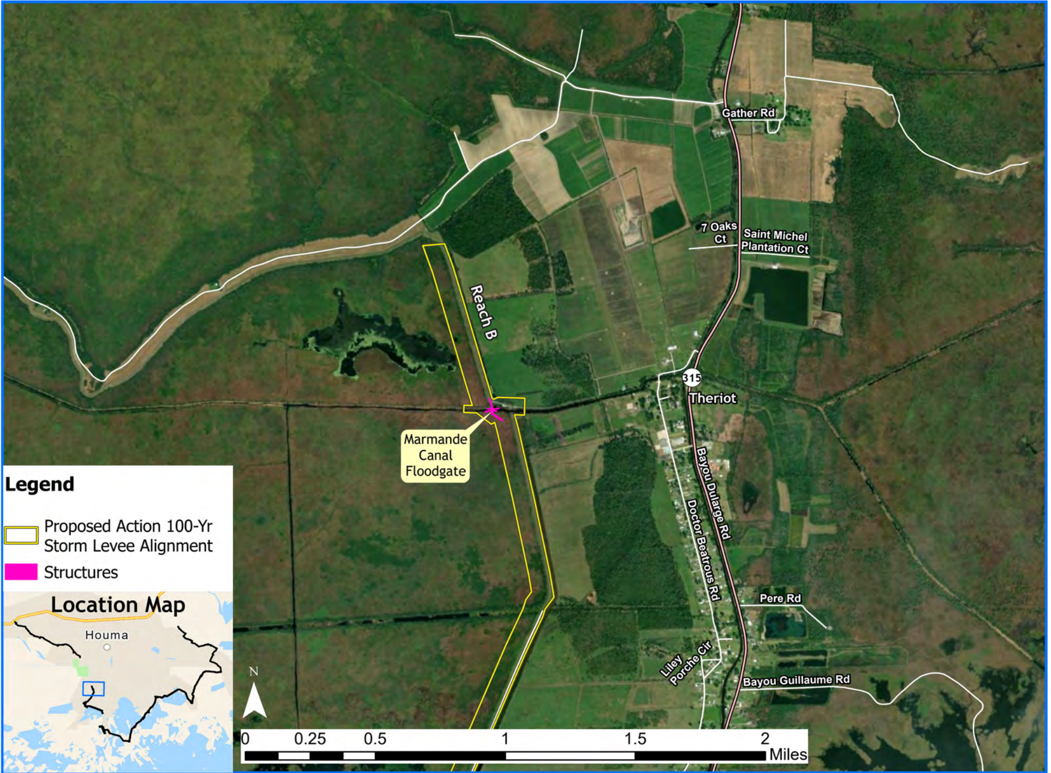
Proposed Action with Structures - Reach B
