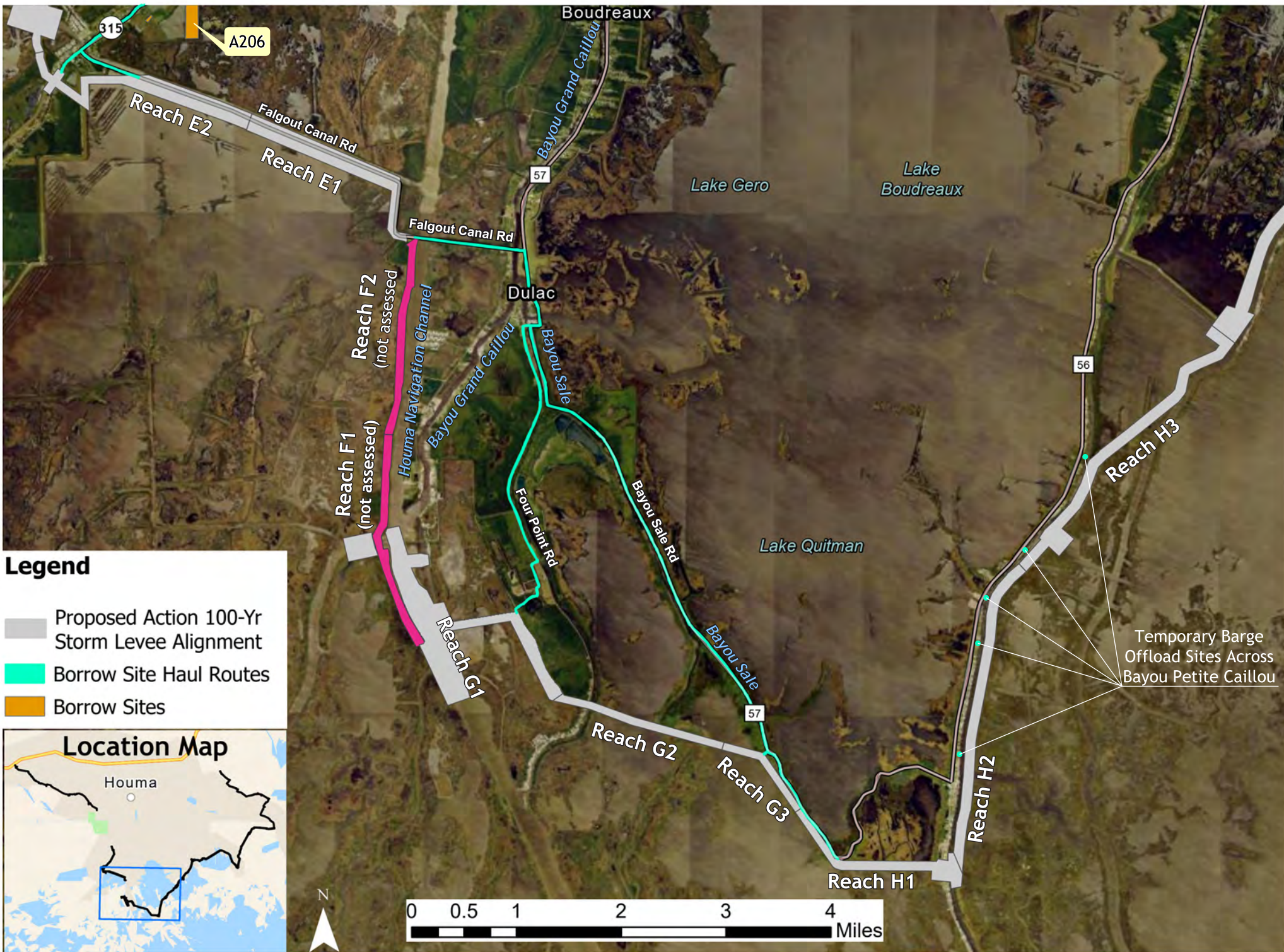
Borrow Sites & Routes - Reaches E and G
