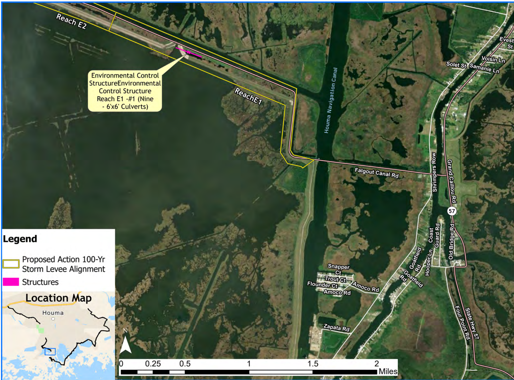
Proposed Action with Structures - Reach E
