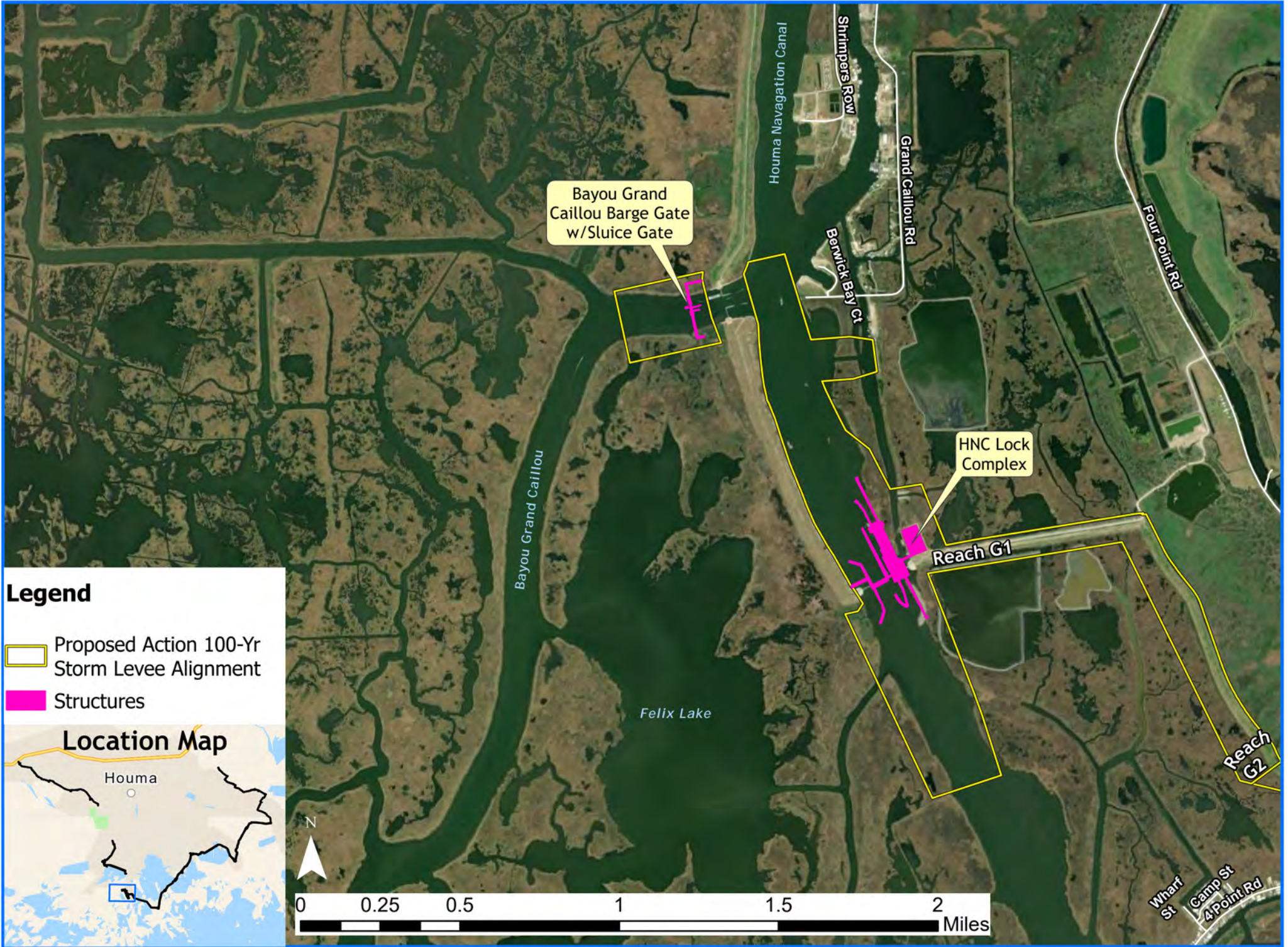
Proposed Action with Structures - Reach G
