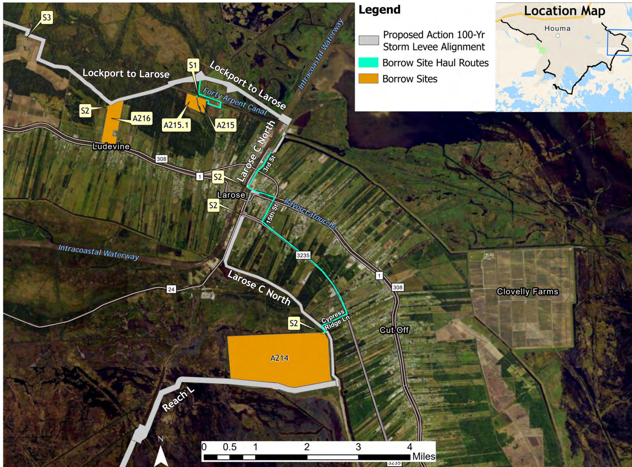
Borrow Sites & Routes - Reaches K, L, Larose C North, and Lockport to Larose
